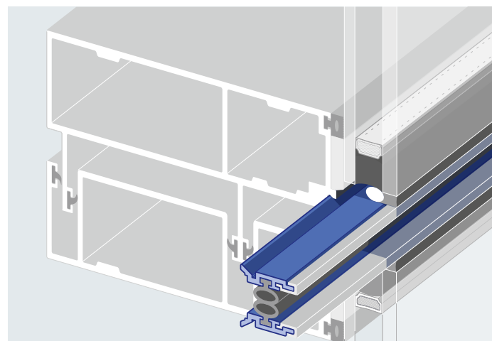
Engineered with Standard profiles: Type: Edge Cover Article Number: 527300
