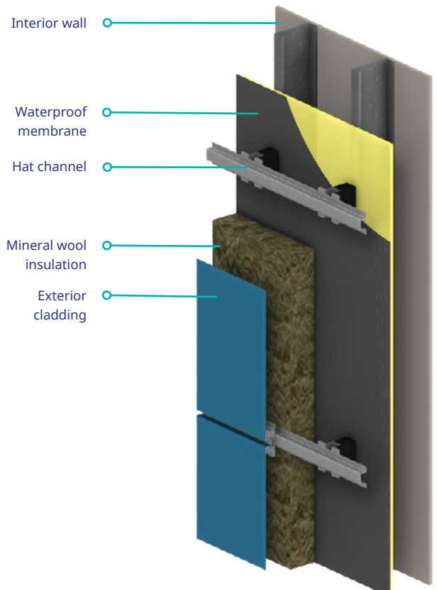
Panel wall system – horizontal application
