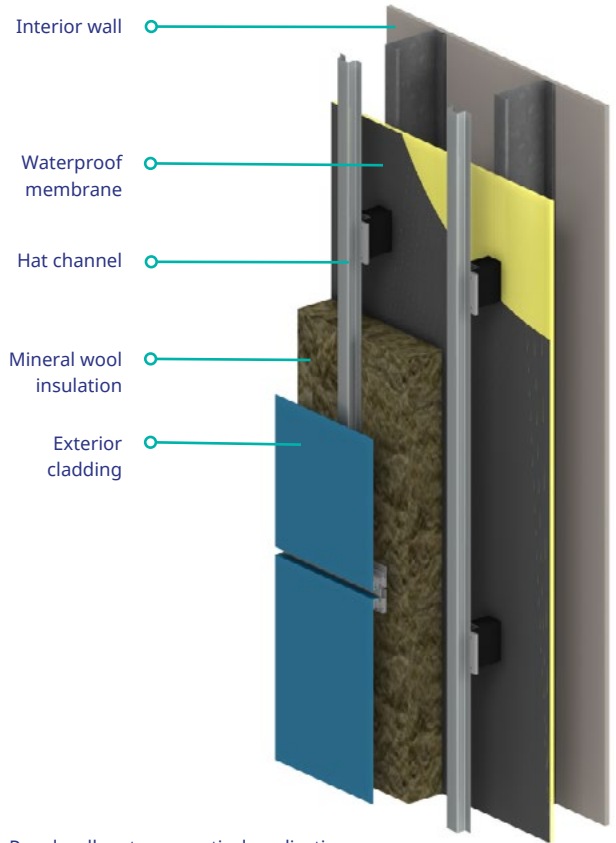
Panel wall system – vertical application
